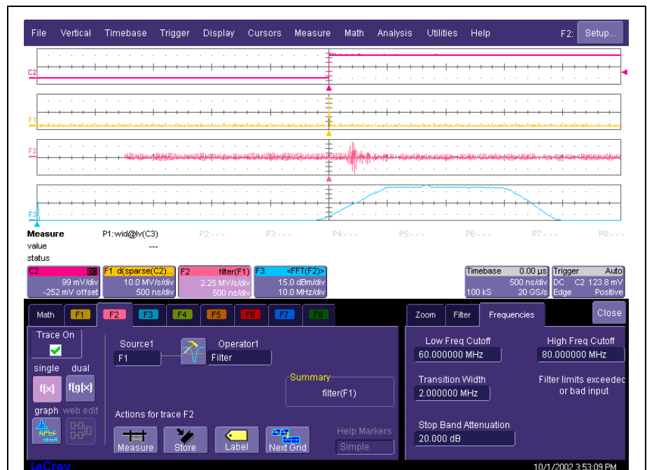
Figure 2 - Filter cutoff frequencies, transition width, and stop band attenuation controls in the DFP2 filter option for the WaveMaster series oscilloscopes
